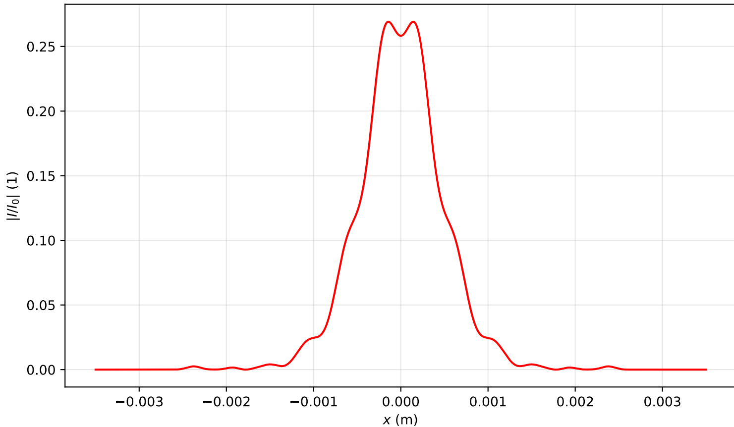
Intensity profile I(x, y = 0, z = 3.025)/I_0 , P_{in}=1.0P_{cr} , artificial time
